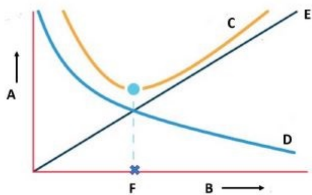
Figure: EOQ model
